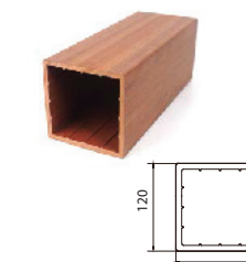
F120C (120X120mm)
