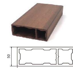
F15050C (150X50mm)
