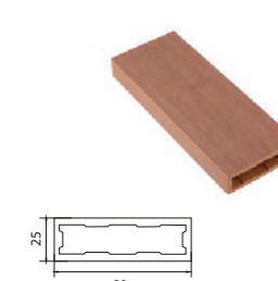
F082C (80X25mm)
