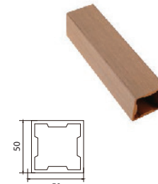
F060C (50X50mm)
