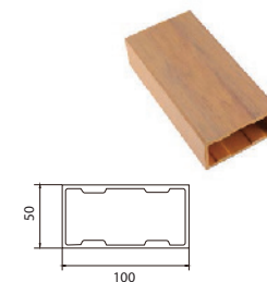
F040C (100X50mm)
